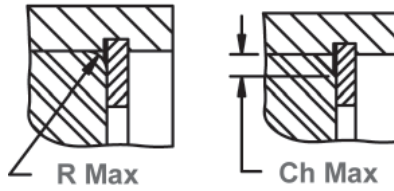
Allowable Corner Radius & Chamfer
