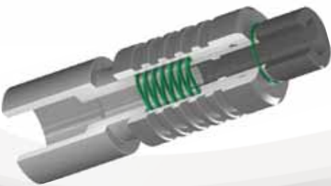
MULTI-TURN WAVE SPRING in Fluid Connector
